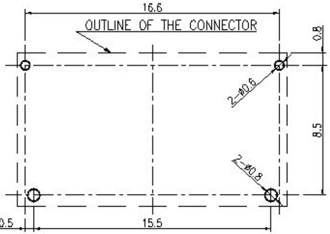
Recommended PCB Layout (UNLESS SPECIFIED DIMENSION TOLERANCE=±0.05)
