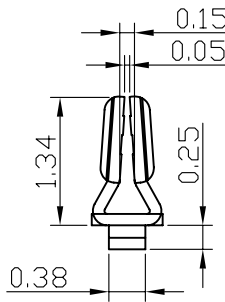
Section C – C
