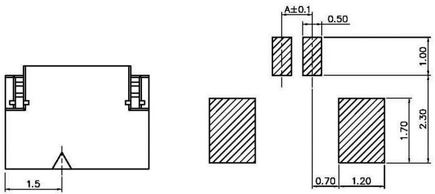
PCB PATTREN LAYOUT
