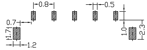
Recommad PCB Layout
