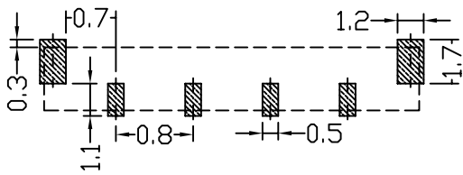
Recommend PCB Layout
