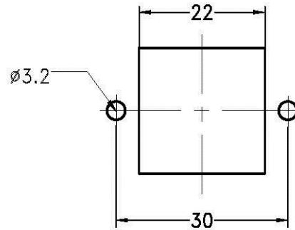
面板开孔图 Panel cut out
