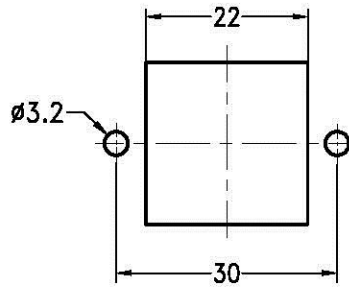
面板开孔图 Panel cut out
