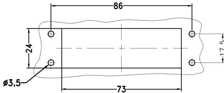
面板开孔图 Panel cut out
