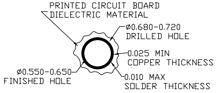
THRU HOLE PLATING SCALE 10:1
