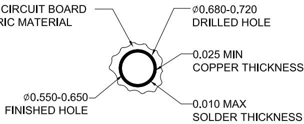
THRU HOLE PLATING SCALE 10:1
