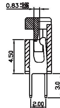
SECTION M-M
