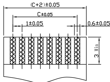
ACCOMMENDED FFC/FPC DIM. THICKNESS 0.3 \pm 0.03 \text{ mm}
