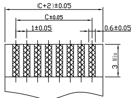
RECOMMENDED FFC/FPC DIM. THICKNESS 0.3±0.03 mm
