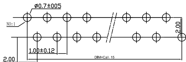
正針線路板 Positive-needle circuit board
