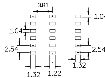
Recommended P.C.Board SMT Layout
