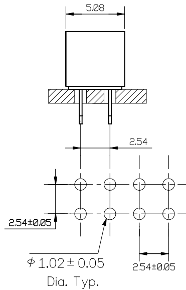
Recommended P.C.Board Hole Layout
