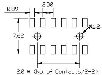
Recommended P.C.Board SMT Layout
