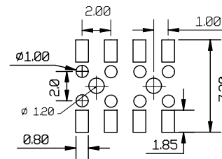
Recommended P.C.Board SMT Layout
