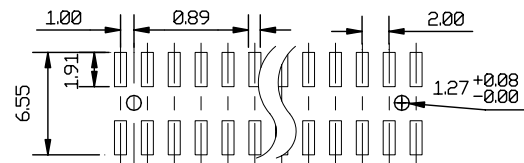
Recommended P.C.Board SMD Layout
