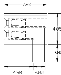
Recommended P.C.Board Hole Layout
