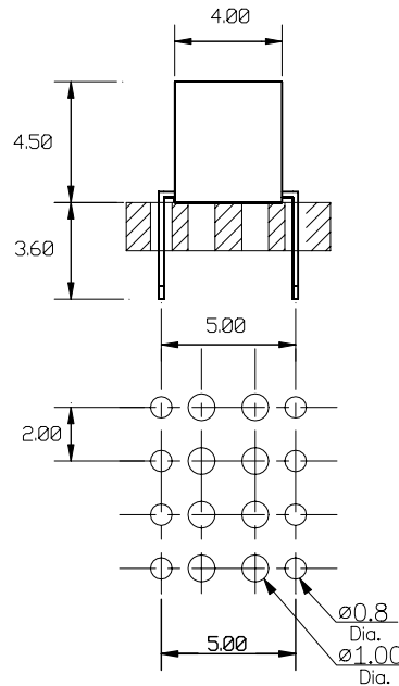
Recommended P.C.Board Hole Layout
