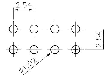
Recommended P.C.Board Hole Layout (Tolerance: ±0.05)
