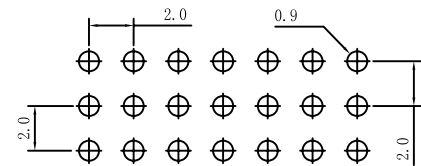
Recommended P.C.B. Layout (Tolerance:0.05mm)
