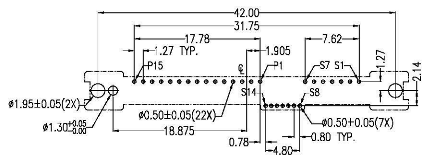
PCB LAYOUT(T=1.60mm) COMPONENT SIDE
