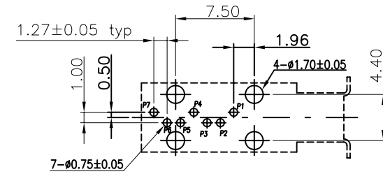
P.C. BOARD MOUNTING DIMENSIONS t=1.60mm PCB TOLERANCE:±0.05
