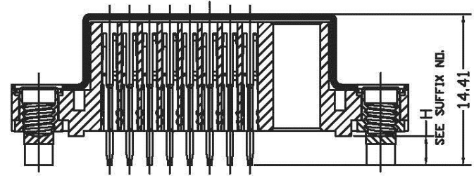
B-B SECTION
