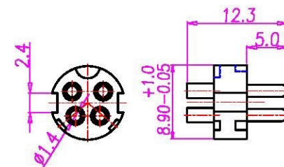
1-1. HOUSING & CONTACT ASSEMBLY
