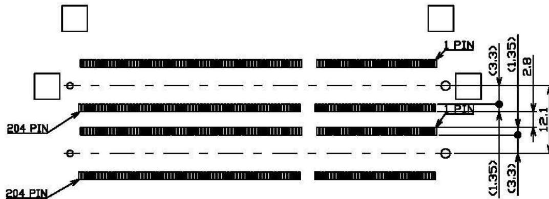
RECOMMENDED MOUNTING P.C. BOARD PATTERN LAYOUT DIM.
