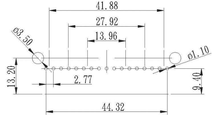
PCB LAYOUT
