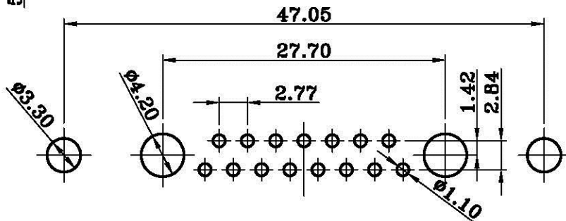
PCB LAYOUT
