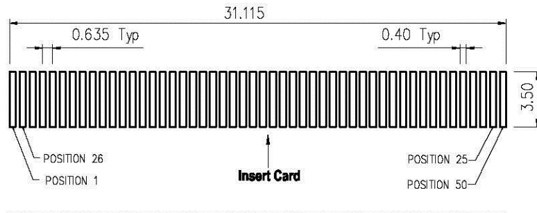
PCB LAYOUT
