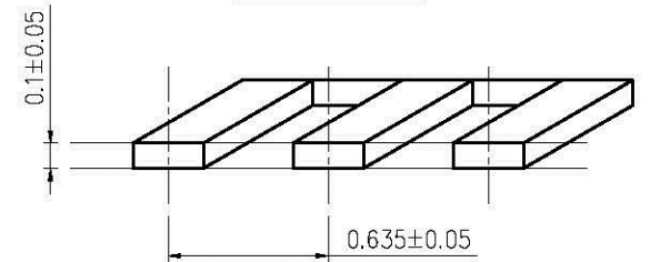
DETAIL "A" 10:1
