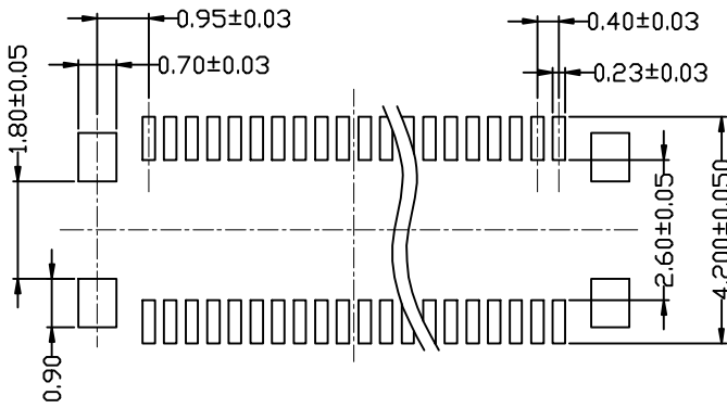
RECOMMENDED PCB LAYOUT CONNECTOR SIDE
