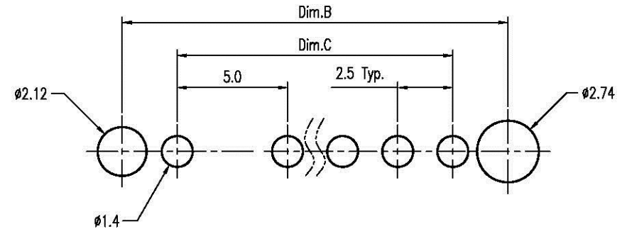
Recommended P.C.B. Layout Layout Tolerance = \pm 0.05 mm
