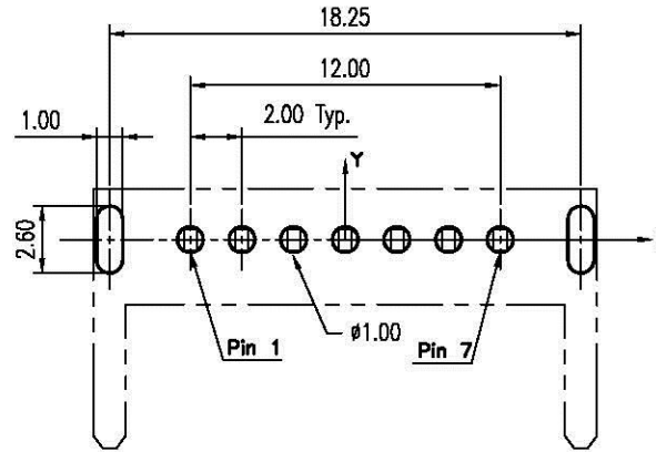
Recommended P.C.B. Layout-1 Layout Tolerance = \pm 0.05 mm
