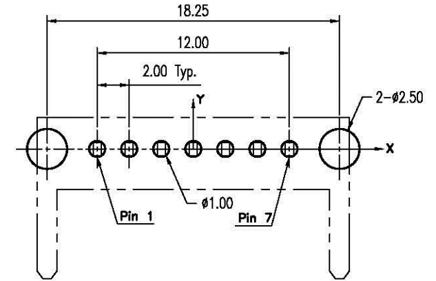
Recommended P.C.B. Layout-2 Layout Tolerance = \pm 0.05 mm
