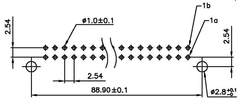
RECOMMENDED P.C.B LAYOUT(TOP VIEW) TOLERANCES: \pm 0.10\text{mm}
