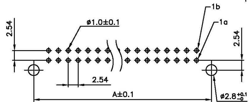
RECOMMENDED P.C.B LAYOUT(TOP VIEW) TOLERANCES: ±0.10mm
