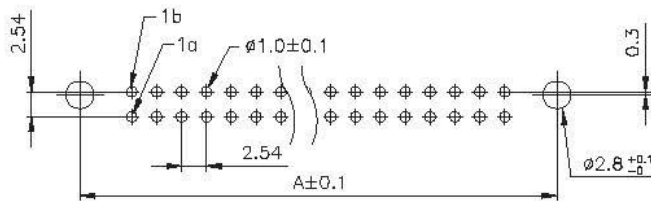
PCB Layout
